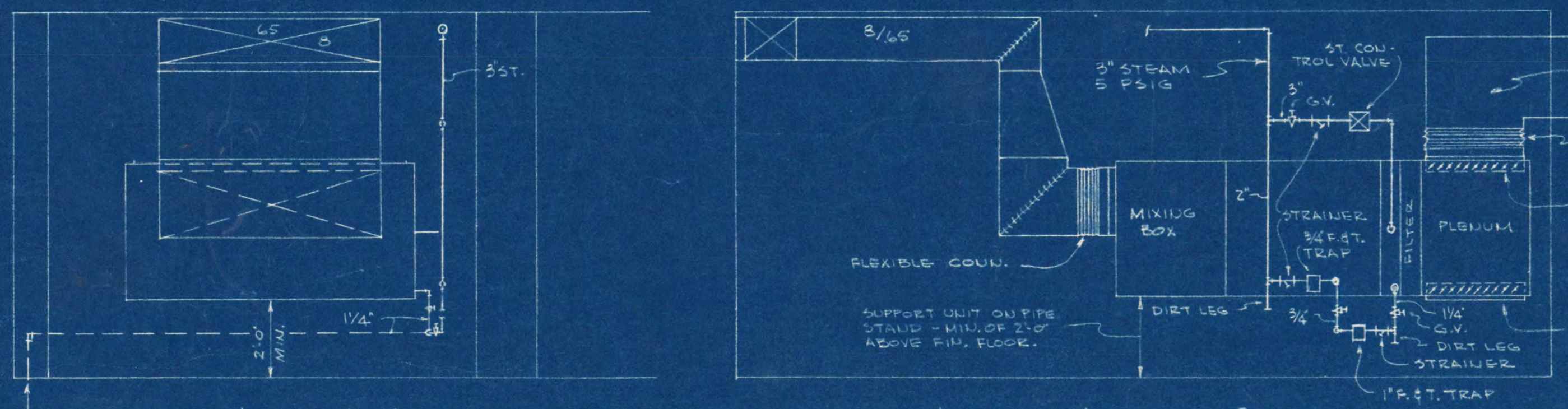
SECTION LOOKING SOUTH DOWN TO TUNNEL SECTION LOOKING EAST RECREATION ROOM VENTILATION UNIT SCALE 3/8" = 1'-0"
