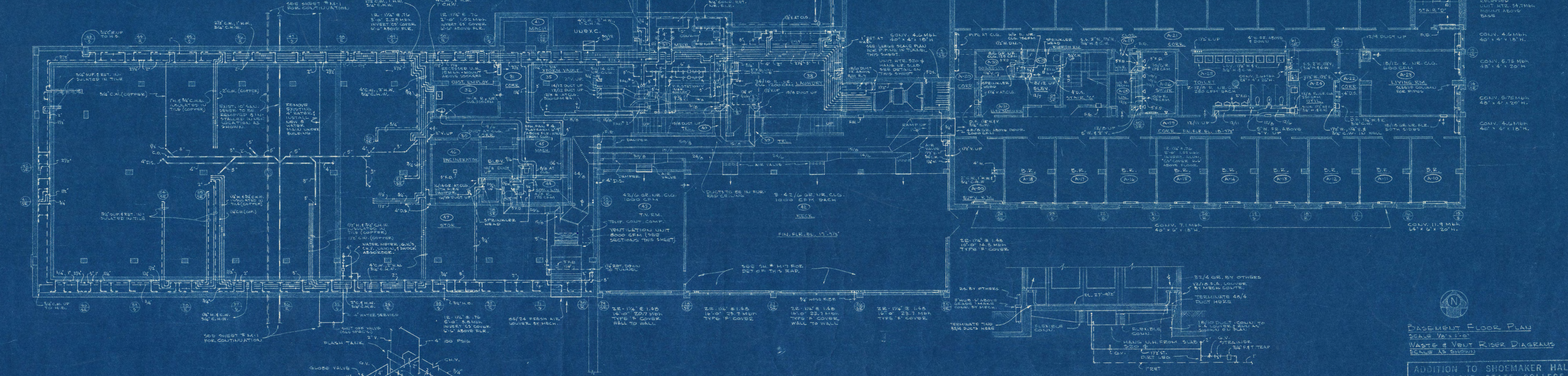
BASEMENT FLOOR PLAN SCALE 1/8" = 1'-0"
