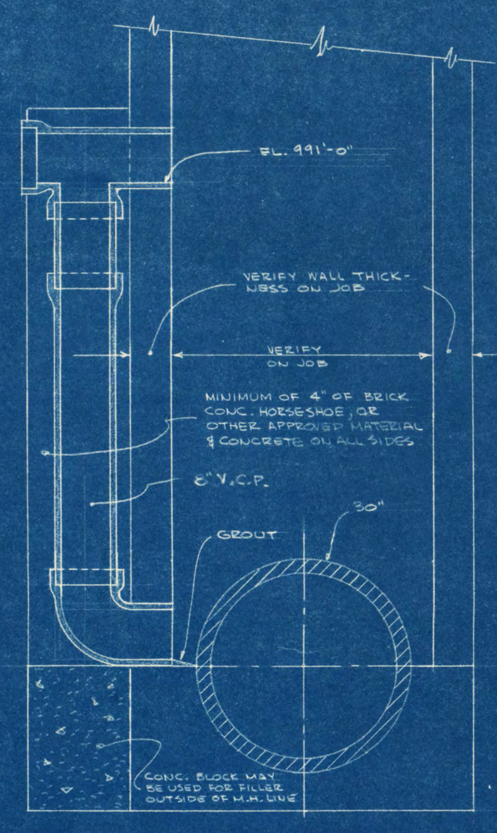
DETAIL OF OUTSIDE DROP PIPE CONSTRUCTION FOR EXIST. MANHOLE NO. 3 SCALE
