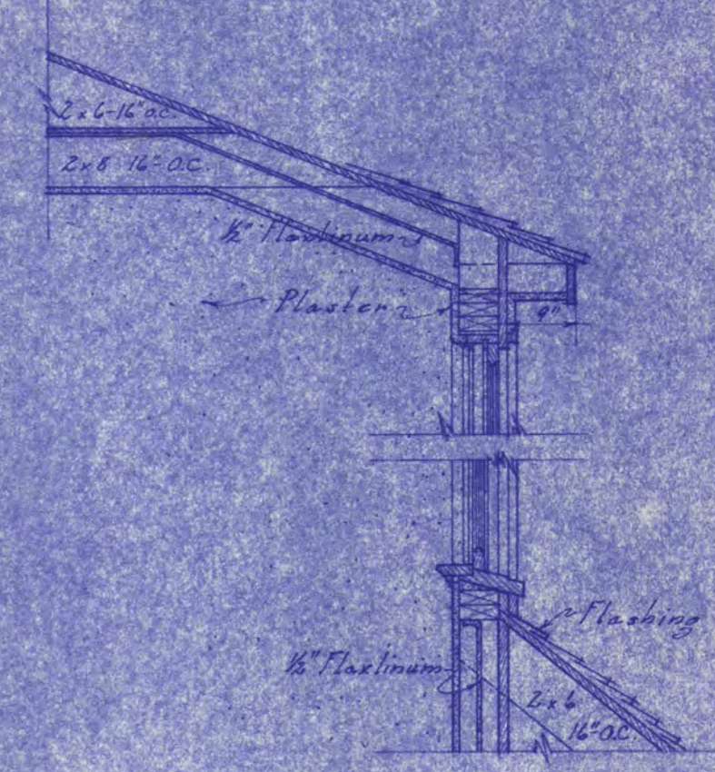
DETAIL OF DORMER-BEDROOM Scale: 1/2"=1'-0"
