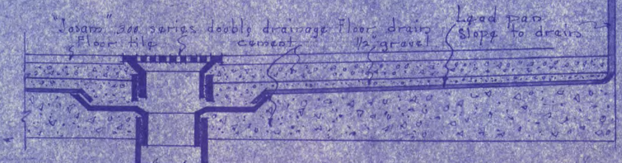
DETAIL SHOWING DRAIN & LEAD PAN FOR SHOWER STALL Lead pan & drain to be installed by plumbing contractor
