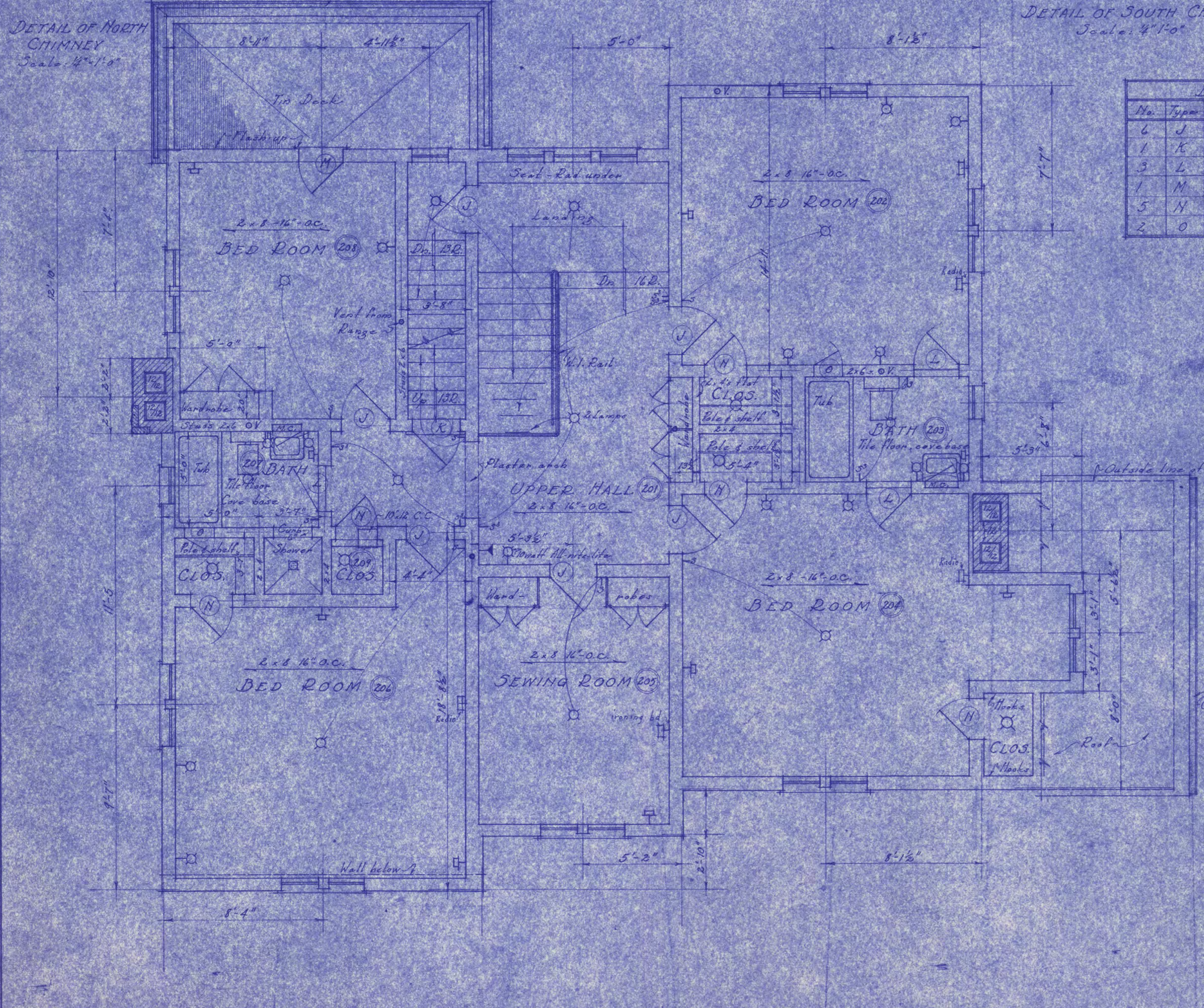
SECOND FLOOR PLAN Scale: 1/8"=1'-0"
