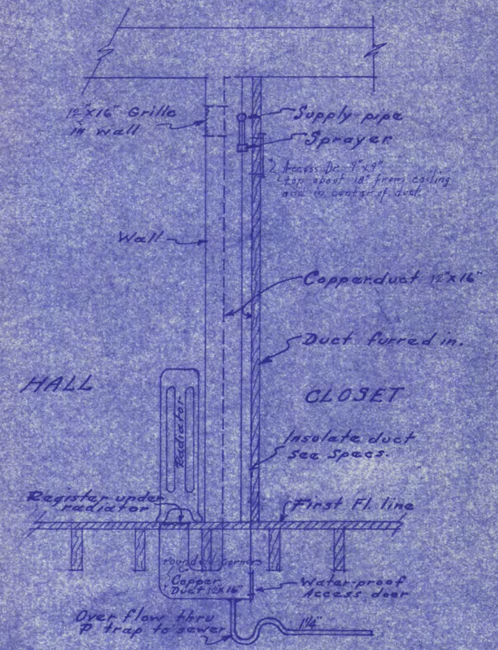
DETAIL OF HUMIDIFYING SYSTEM ON FIRST FL. Scale 1/2" = 1'-0"
