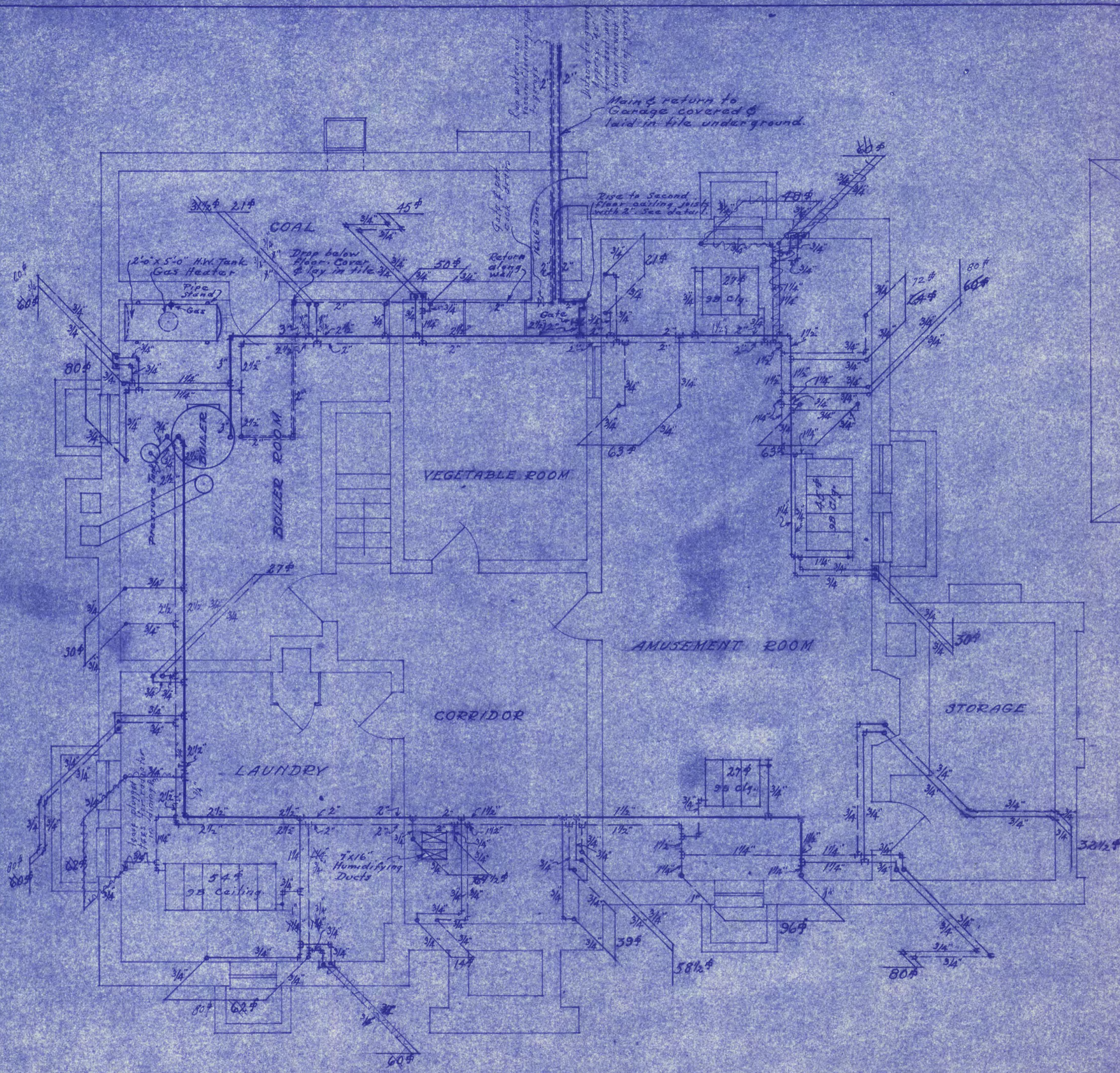
BASEMENT PIPING PLAN Scale 1/4" = 1'-0"
