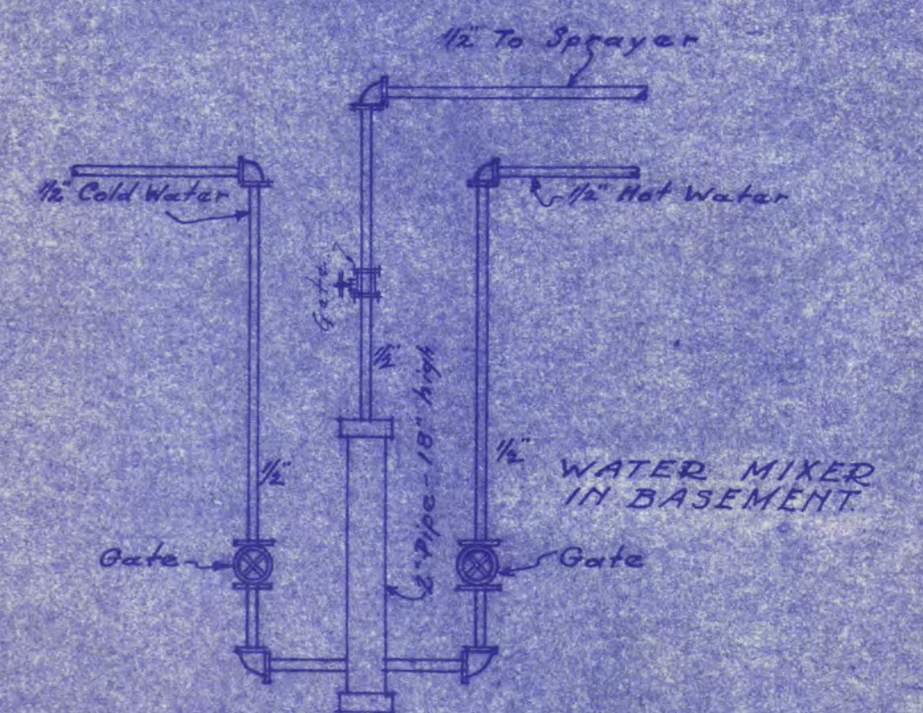
DETAIL OF WATER MIXER FOR HUMIDITY SPRAY No Scale
