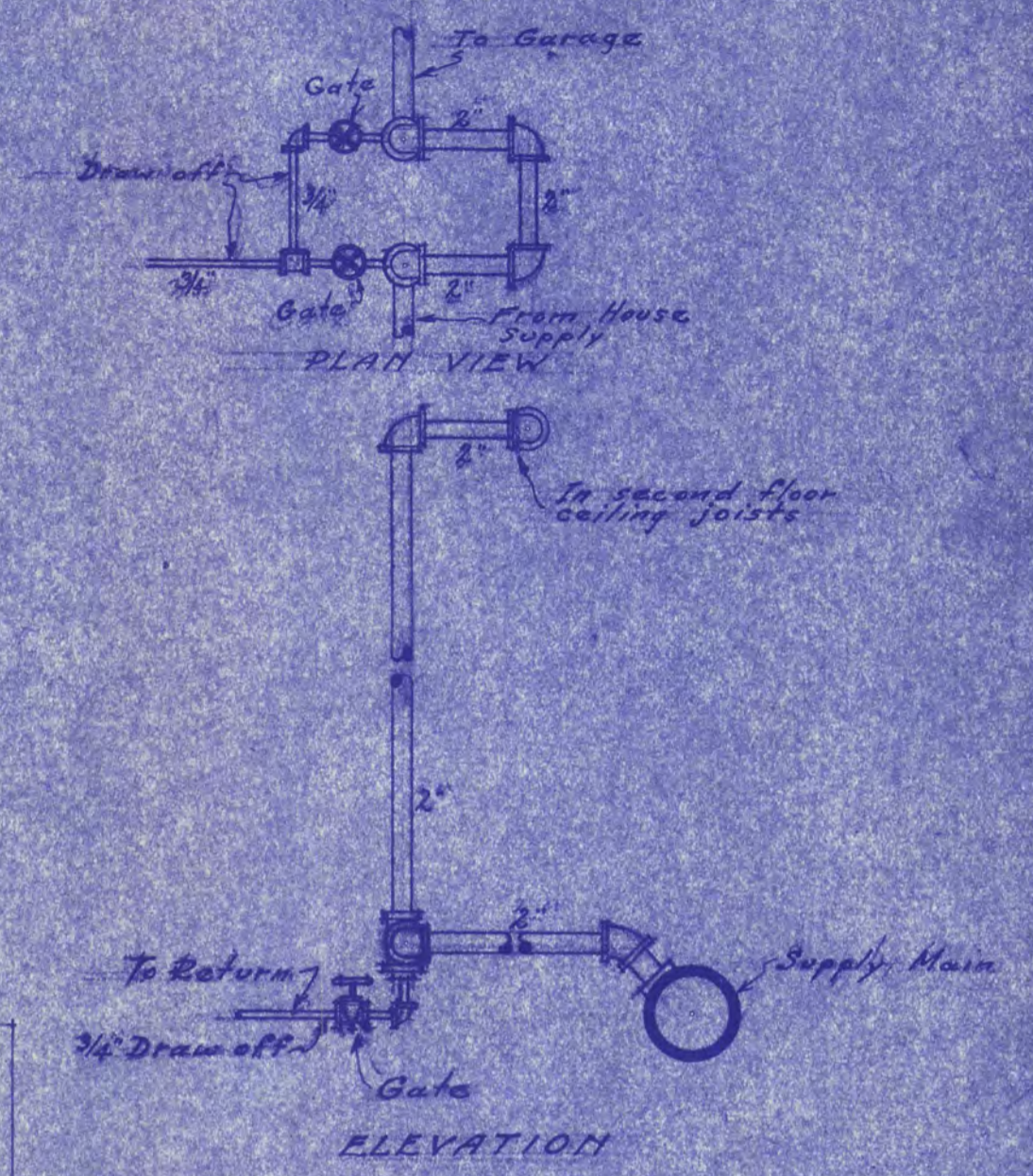
DETAIL OF RISERS FOR GARAGE MAIN SUPPLY No. Scale
