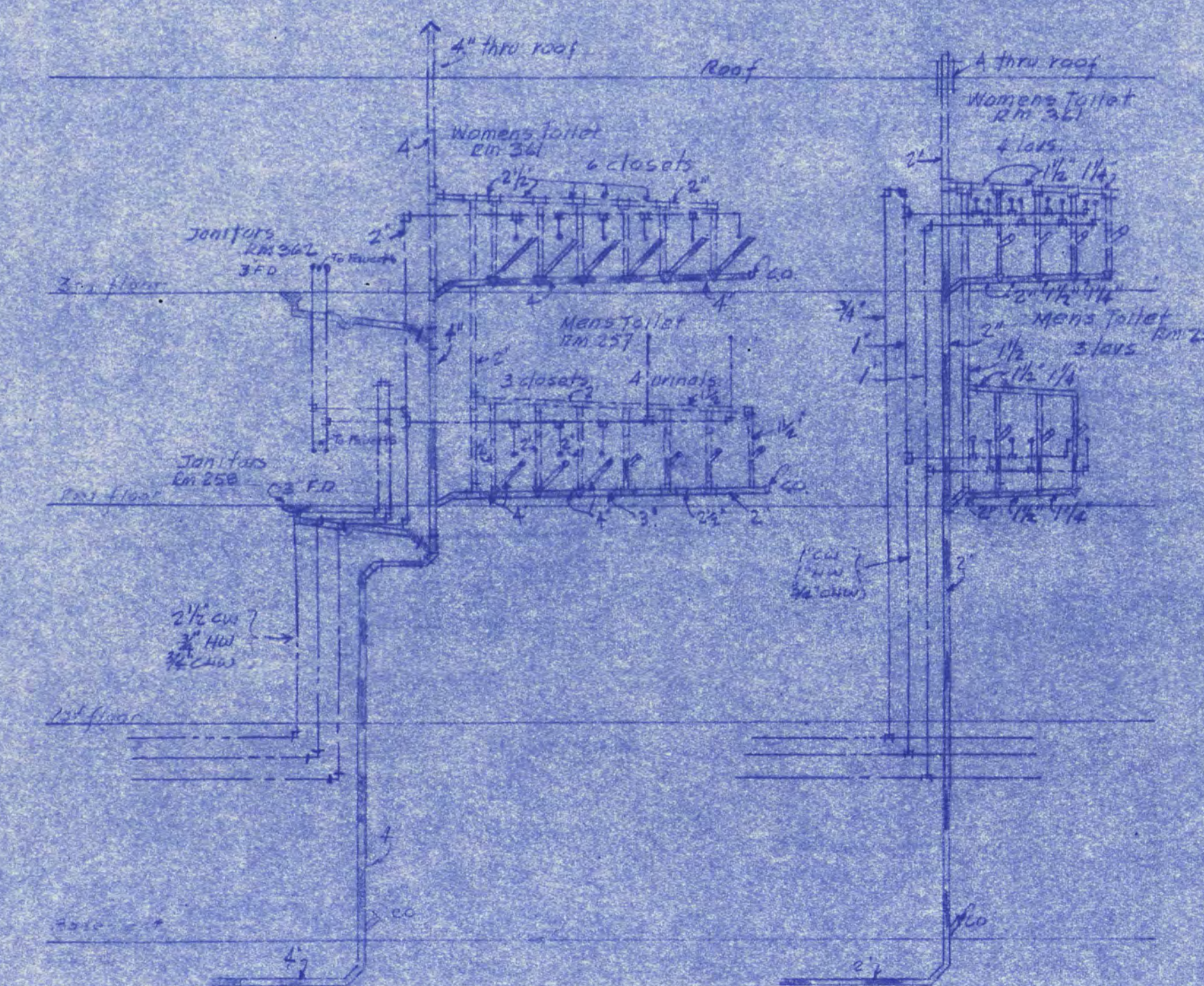
PLUMBING RISER DIAGRAM TOILET ROOMS 257-321 No SCALE
