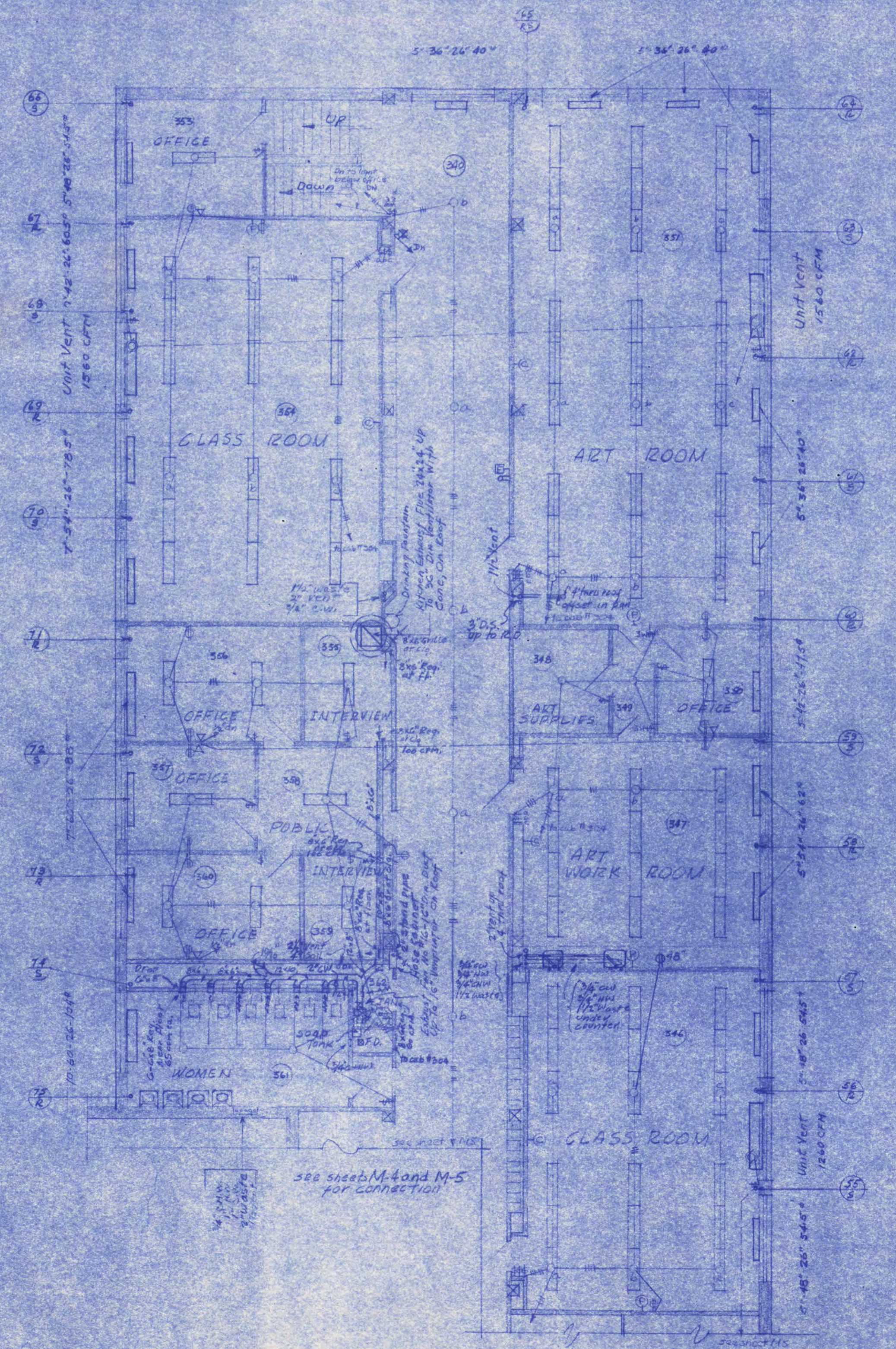
PART THIRD FLOOR PLAN SCALE 1/8" = 1'-0"
