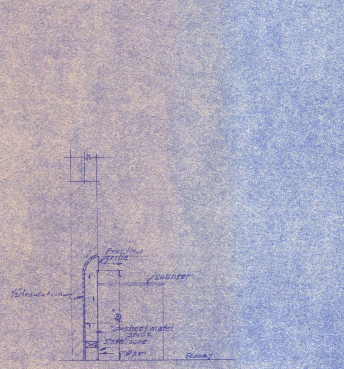
DETAIL OF SPECIAL SHEET METAL CABINET FOR RADIATORS 1ST FLOOR SHOP SECTION SCALE 1/2" = 1'-0"
