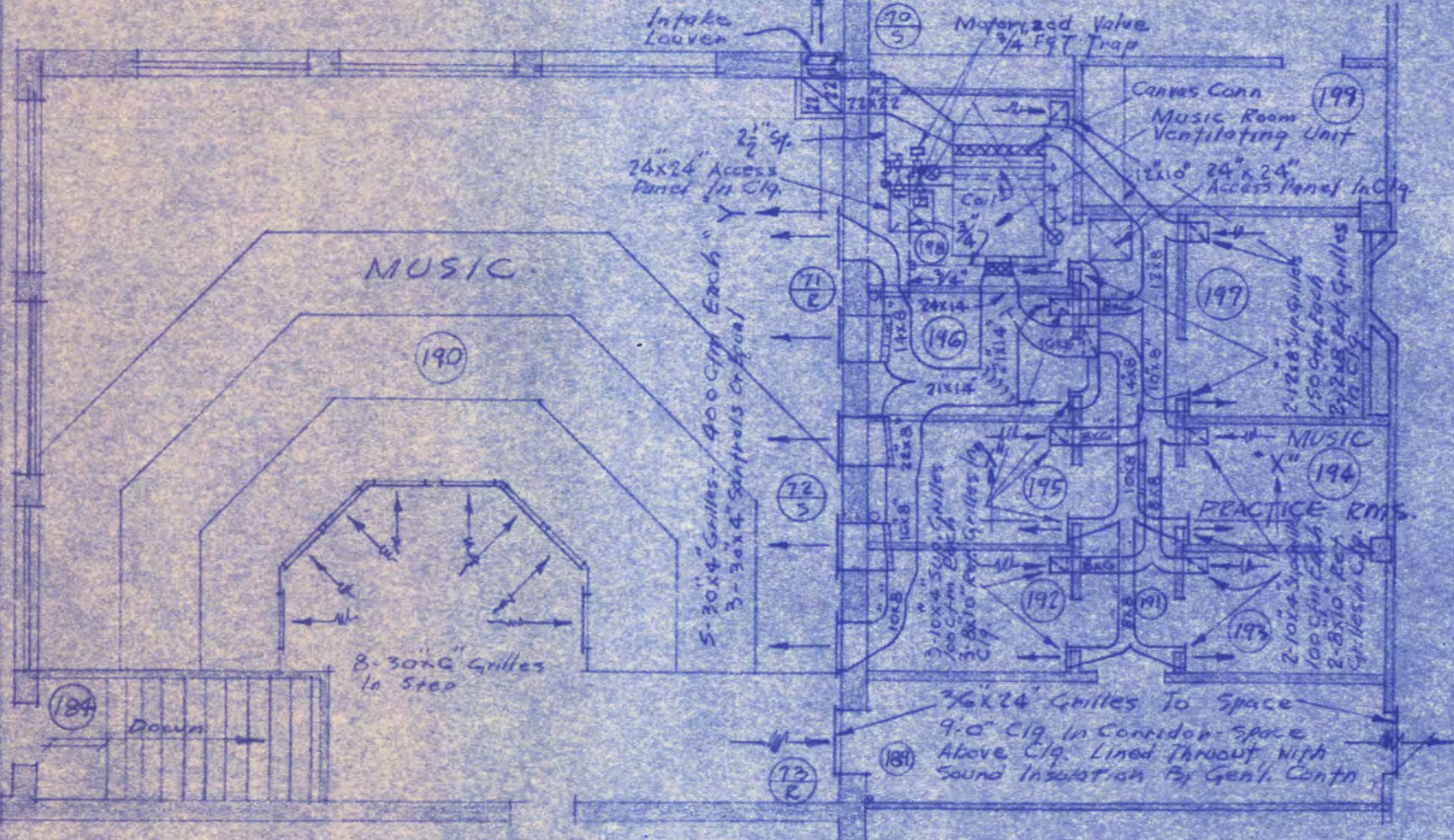
PLAN SCALE 1/8" = 1'-0"
