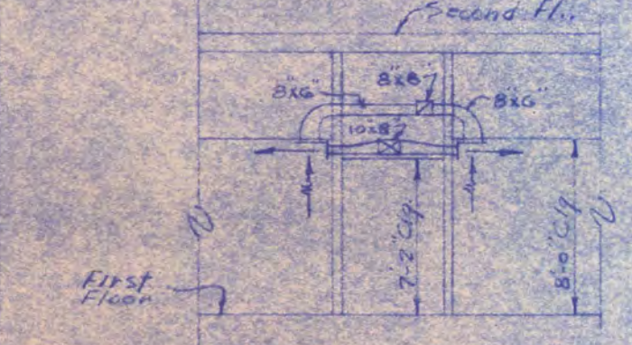
SECTION XX SCALE 1/8" = 1'-0"
