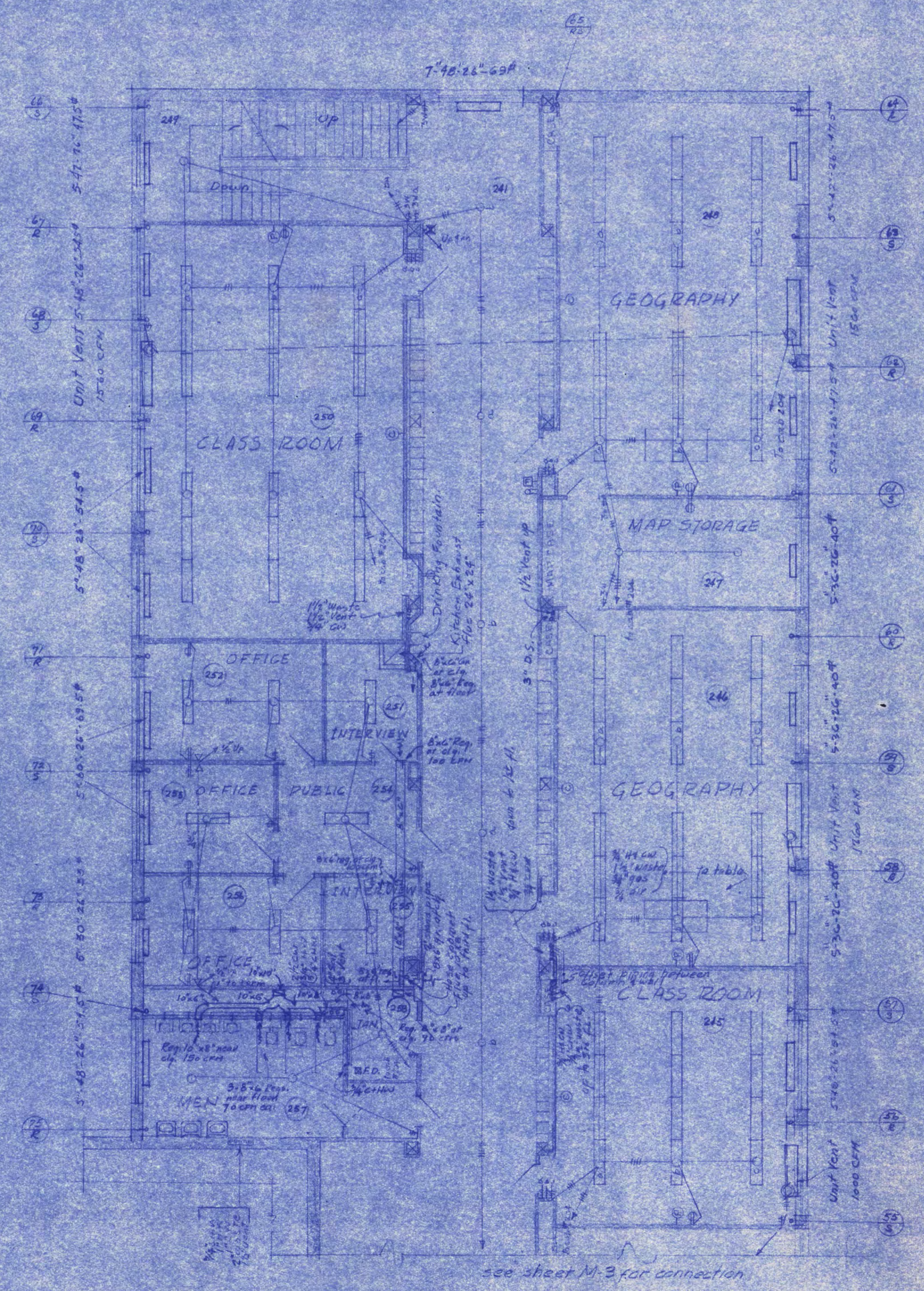
PART SECOND FLOOR PLAN SCALE 1/8" = 1'-0"
